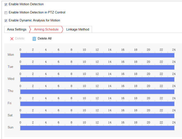
Figure 5-12 Arming Schedule
