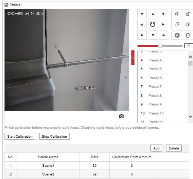
Figure 5-40 Rapid Focus
