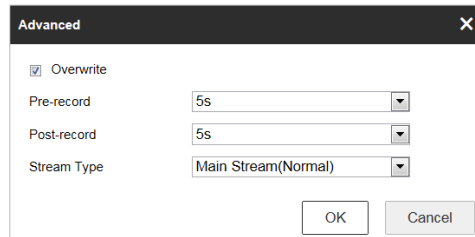
Figure 5-2 Record Parameters
