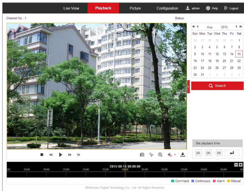
Figure 4-17Figure 4-13 Playback Interface
