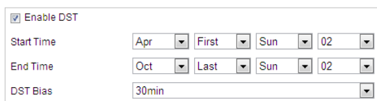
Figure 6-46 DST Settings
