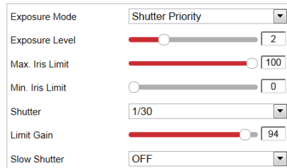
Figure 6-25 Manual Shutter
