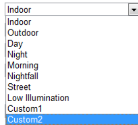
Figure 6-39 Linked Scene
