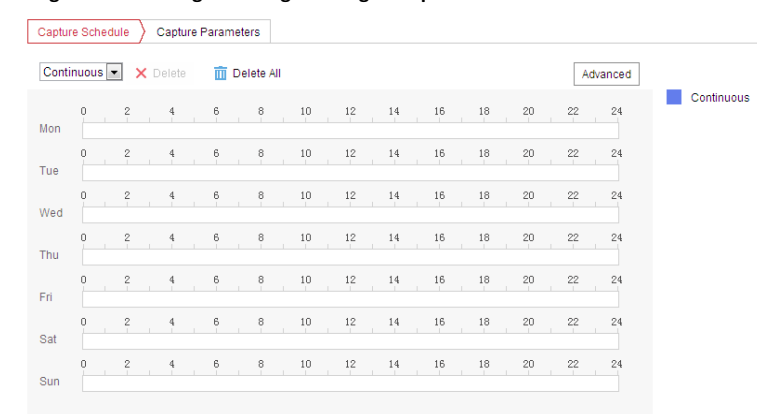
Figure 5-3 Snapshot Settings
