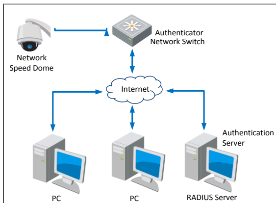
Figure 6-17 Protected LAN
