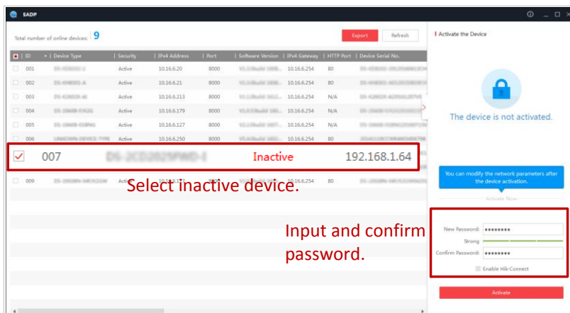
Figure 2-4 SADP Interface
