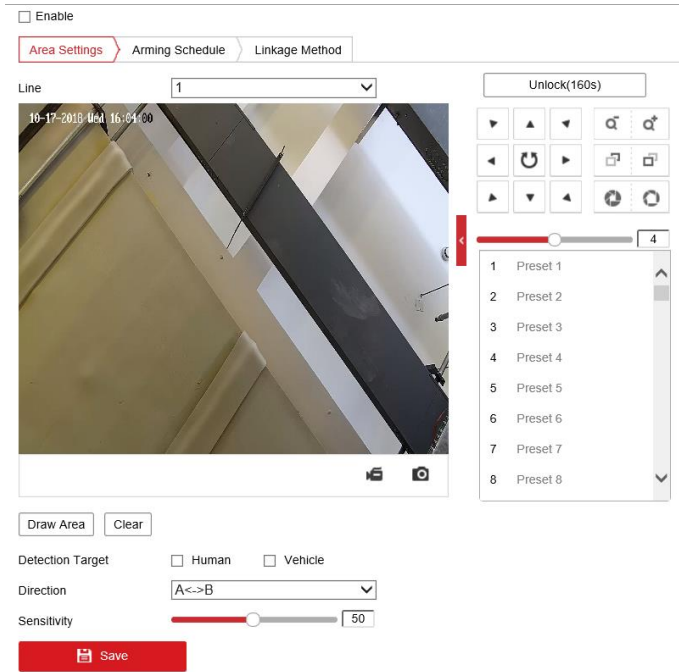
Figure 5-24 Configuring Line
