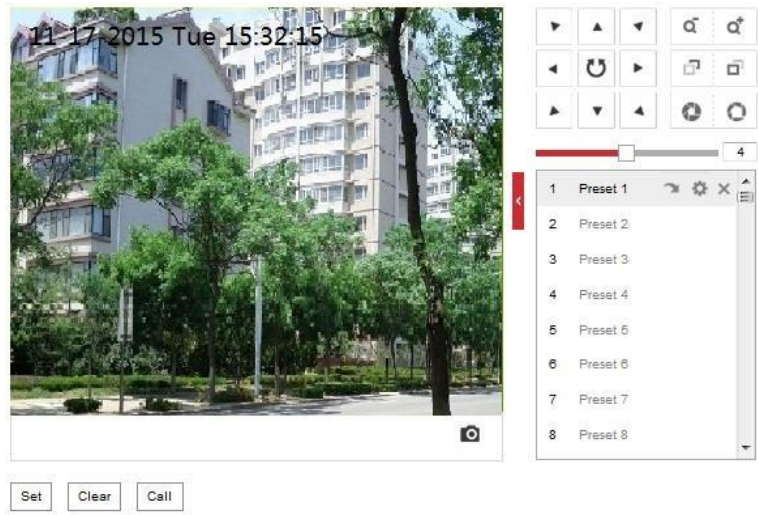
Figure 5-30 PTZ Configuration
