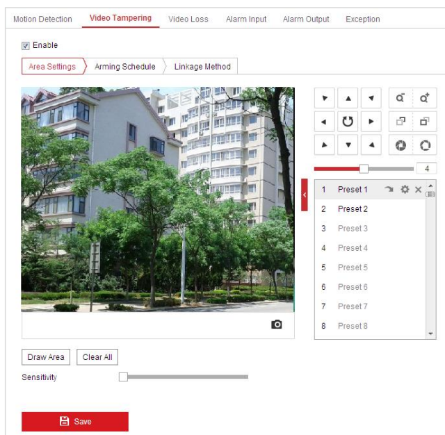
Figure 5-16 Tampering Alarm
