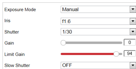
Figure 6-26 Manual Mode
