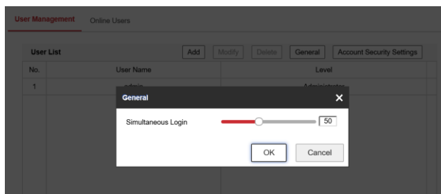
Figure 6-60 Simultaneous Login
