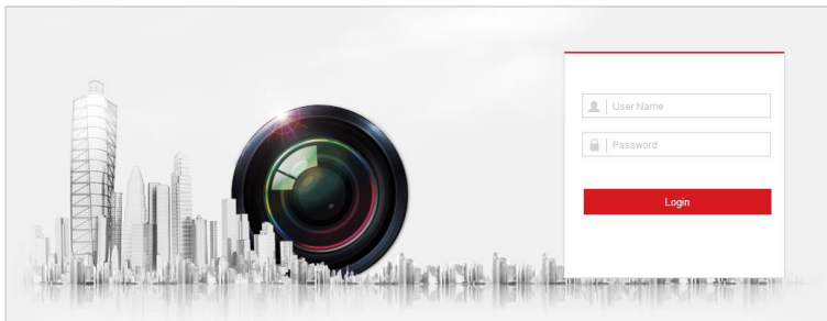
Figure 3-1 Login Interface
