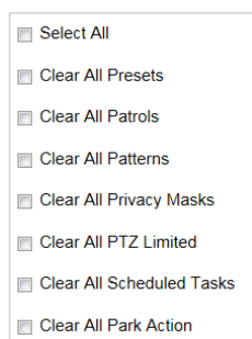
Figure 5-36 Clear Config
