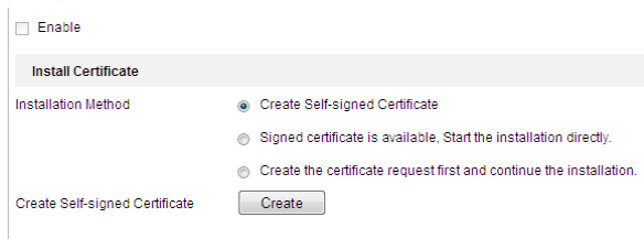
Figure 6-13 Create Certificate
