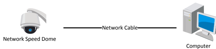
Figure 2-1 Connecting Directly
